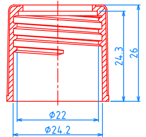
(28/400) CAP, P=1"x6 TPI
