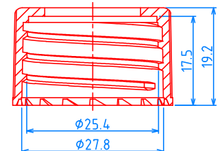
(28/410) CAP, P=1"x6 TPI
