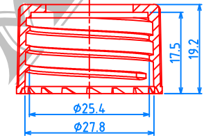
(28/415) CAP, P=1"x6 TPI
