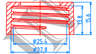
(28/410) CAP, P=1"x6 TPI
