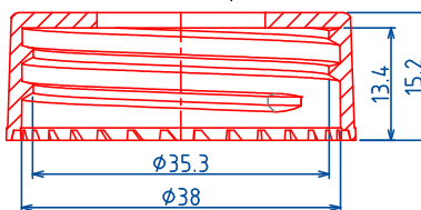
(38/400) (高)CAP ,P=1"x6TPI
