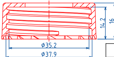
(38/400) (高)CAP ,P=1"x6TPI
