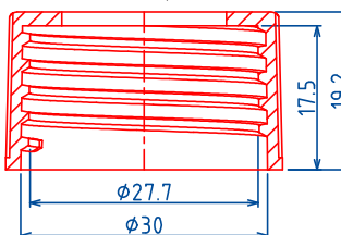
(30/400)CAP ,P=1"x8TPI
