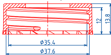
(38/400) (中)CAP ,P=1"x6TPI
