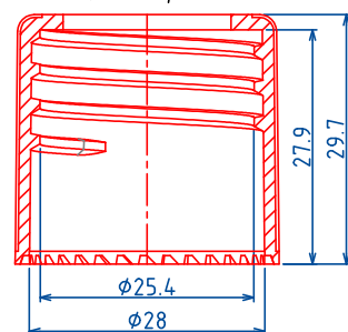
(28/415)CAP ,P=1"x6TPI
