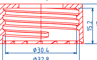
(33/410)CAP ,P=1"x6TPI
