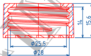
(28/410)CAP ,P=1"x6TPI
