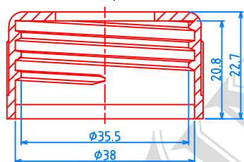
(38/410) CAP, P=1"x6 TPI
