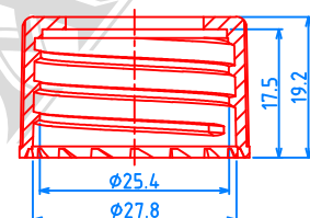
(28/415) CAP, P=1"x6 TPI
