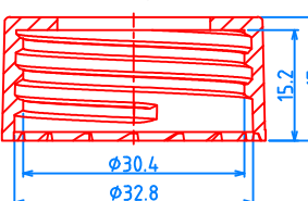
(33/410) CAP, P=1"x6 TPI
