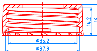
(38/400) (高) CAP, P=1"x6 TPI
