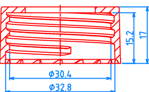
(33/410) CAP, P=1"x6 TPI
