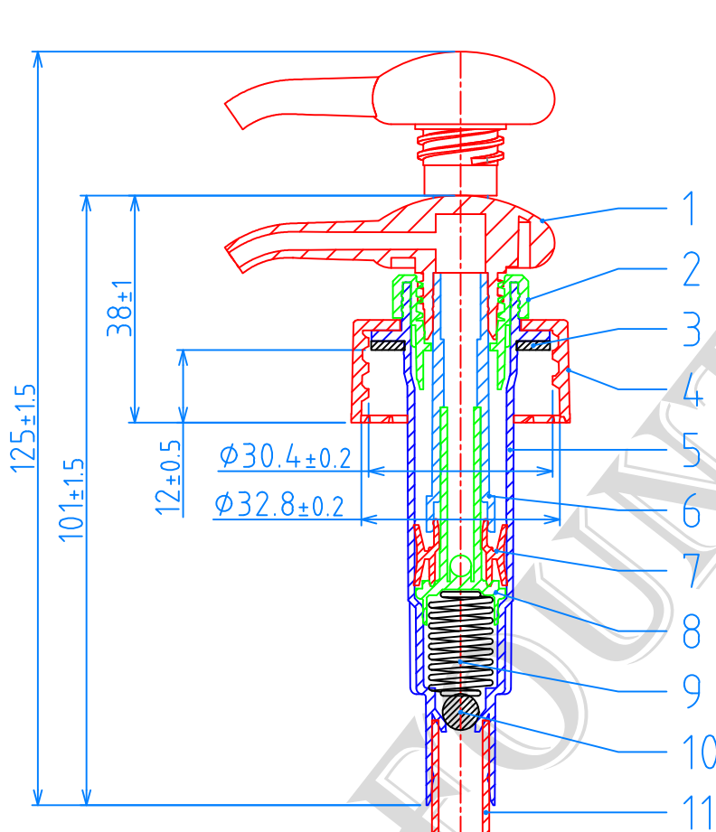
(38/410) CAP, P=1"x6 TPI
