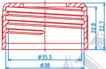
(38/410) CAP, P=1"x6 TPI
