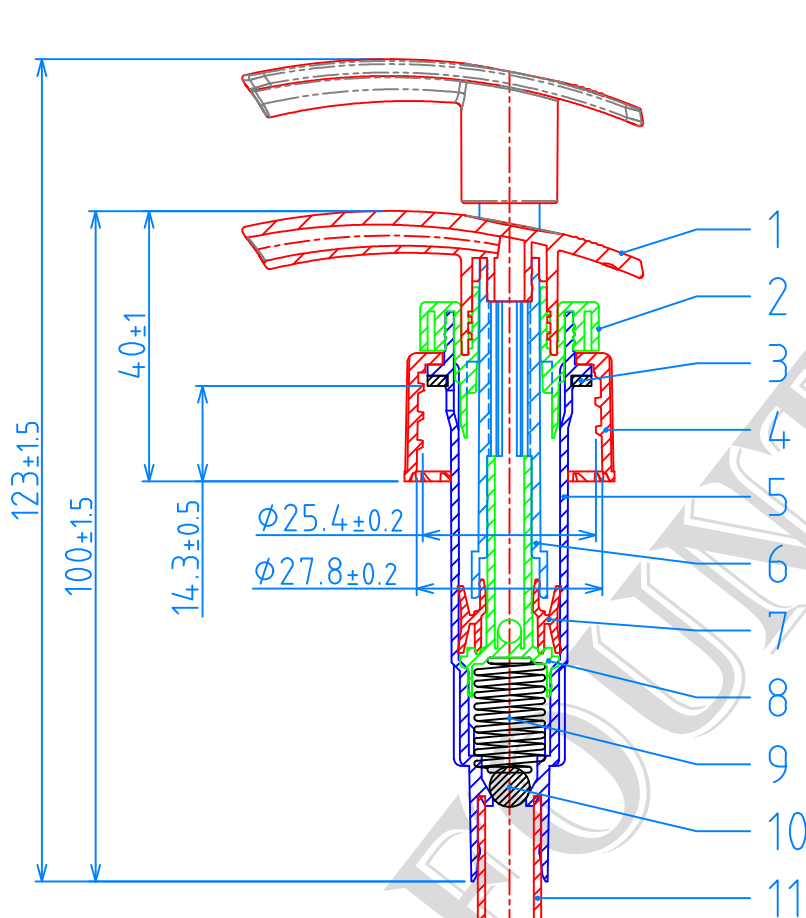
(38/410) CAP , P=1"x6 TPI
