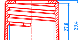
(28/415) CAP, P=1"x6 TPI
