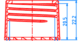
(28/水胚) CAP, P=1"x8 TPI
