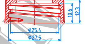
(28/400) CAP, P=1"x6 TPI
