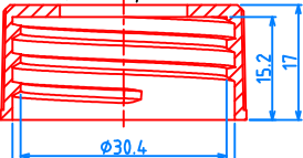
(33/410) CAP, P=1"x6 TPI
