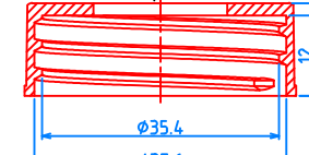
(38/400) CAP, P=1"x6 TPI (低)
