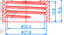
(28/410) CAP, P=1"x6 TPI
