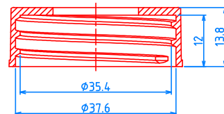
(38/400) CAP, P=1"x6 TPI (低)
