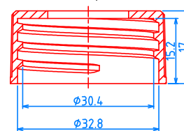
(33/410) CAP, P=1"x6 TPI
