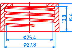
(28/410) CAP, P=1"x6 TPI
