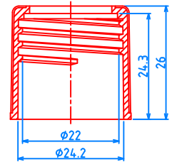
(28/400) CAP, P=1"x6 TPI
