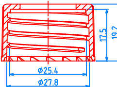
(28/410) CAP, P=1"x6 TPI
