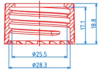
(28/410) CAP , P=1"x6 TPI
