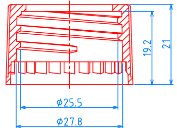
(28/410TR) CAP , P=1"x6 TPI
