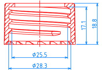
(28/410TR) CAP , P=1"x6 TPI
