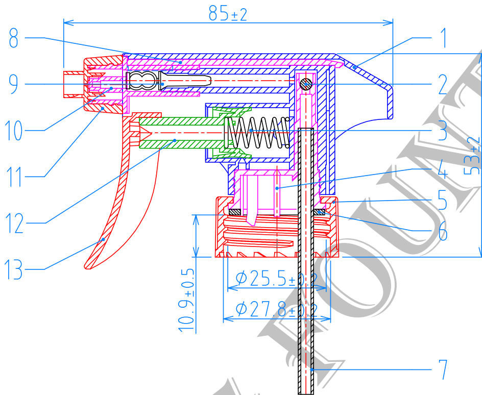
(28/410TR) CAP , P=1"x6 TPI
