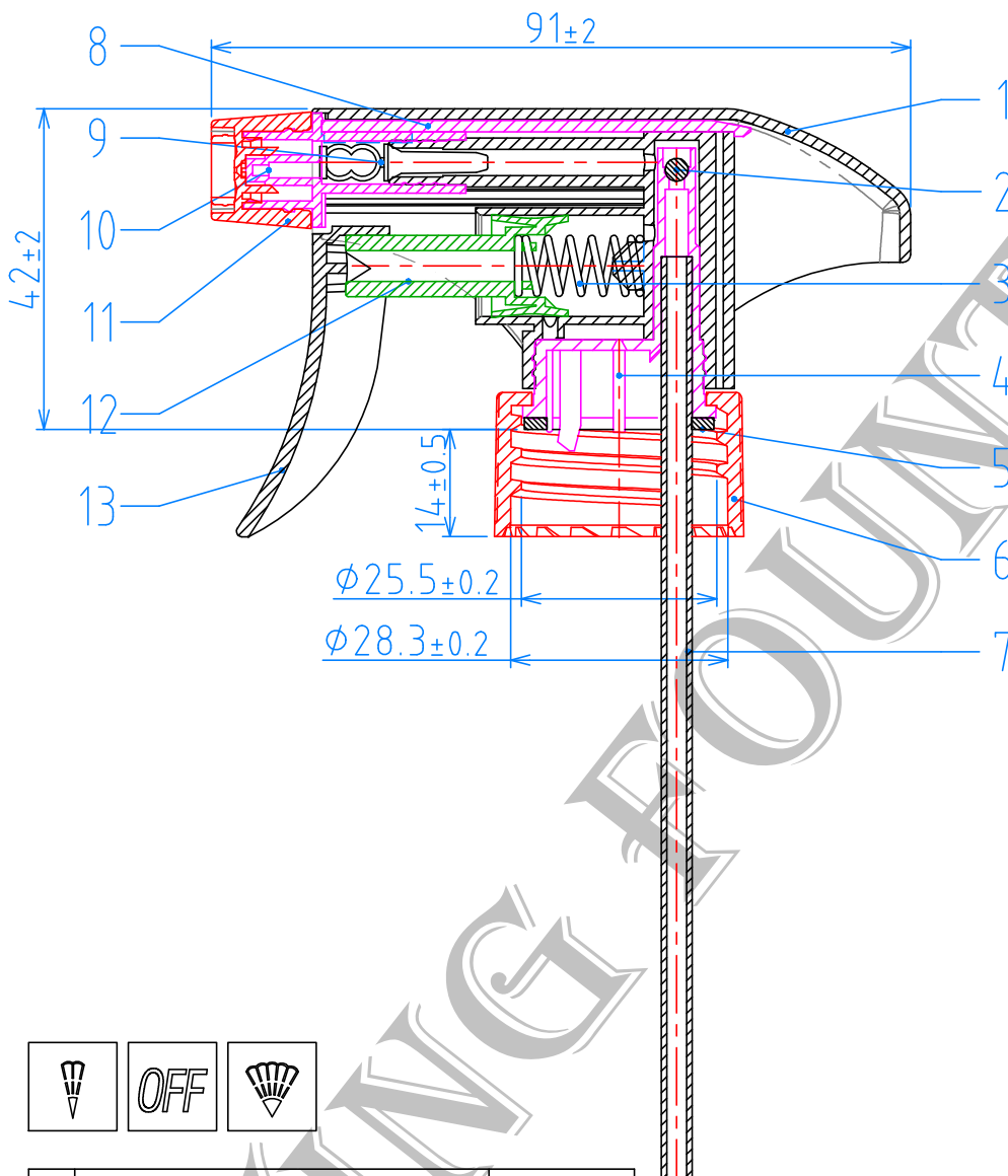
(28/410TR) CAP ,P=1"x6TPI
