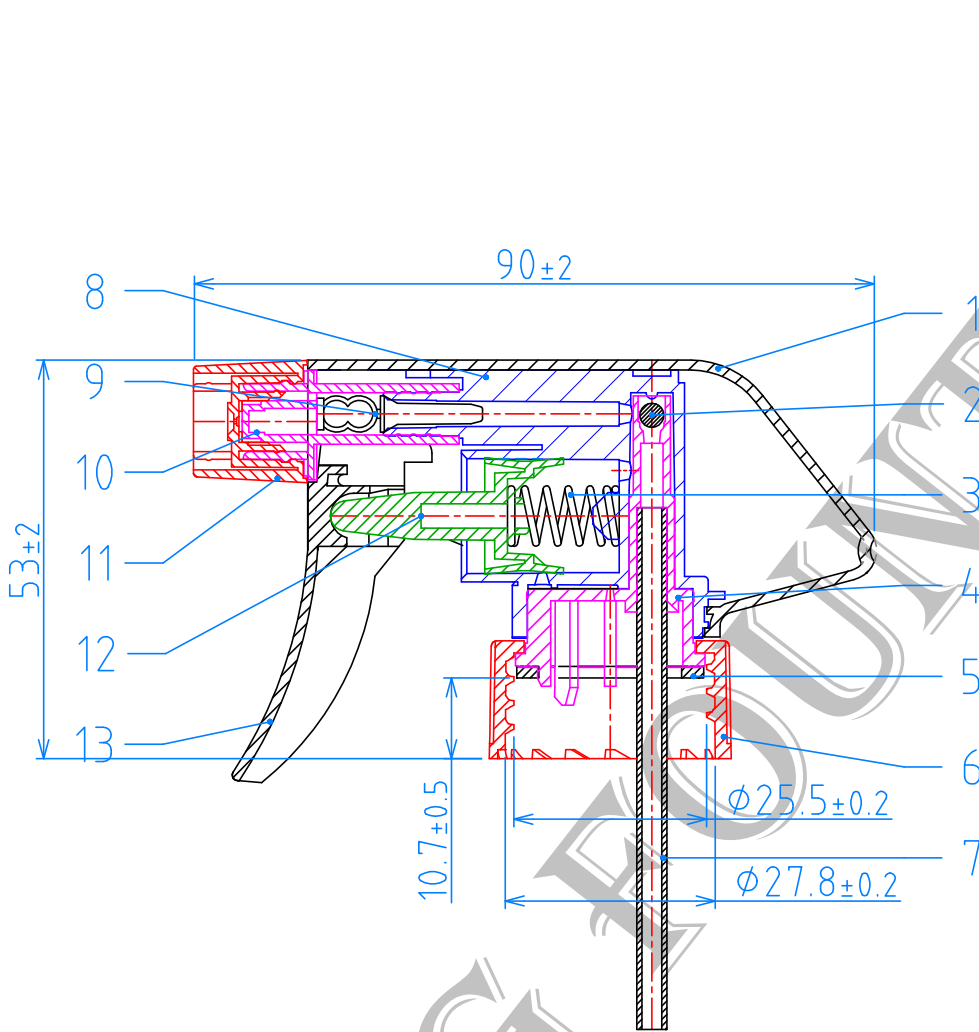
(28/410TR) CAP , P=1"x6 TPI
