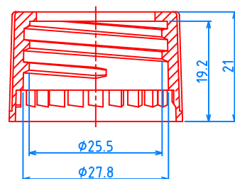
(28/410TR) CAP , P=1"x6 TPI
