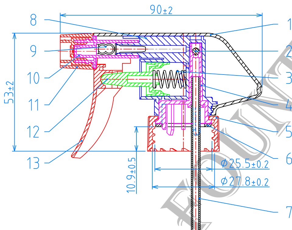
(28/410TR) CAP , P=1"x6 TPI
