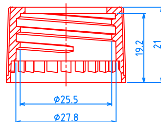
(28/410TR) CAP , P=1"x6 TPI
