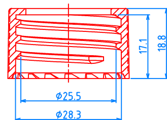
(28/410) CAP , P=1"x6 TPI
