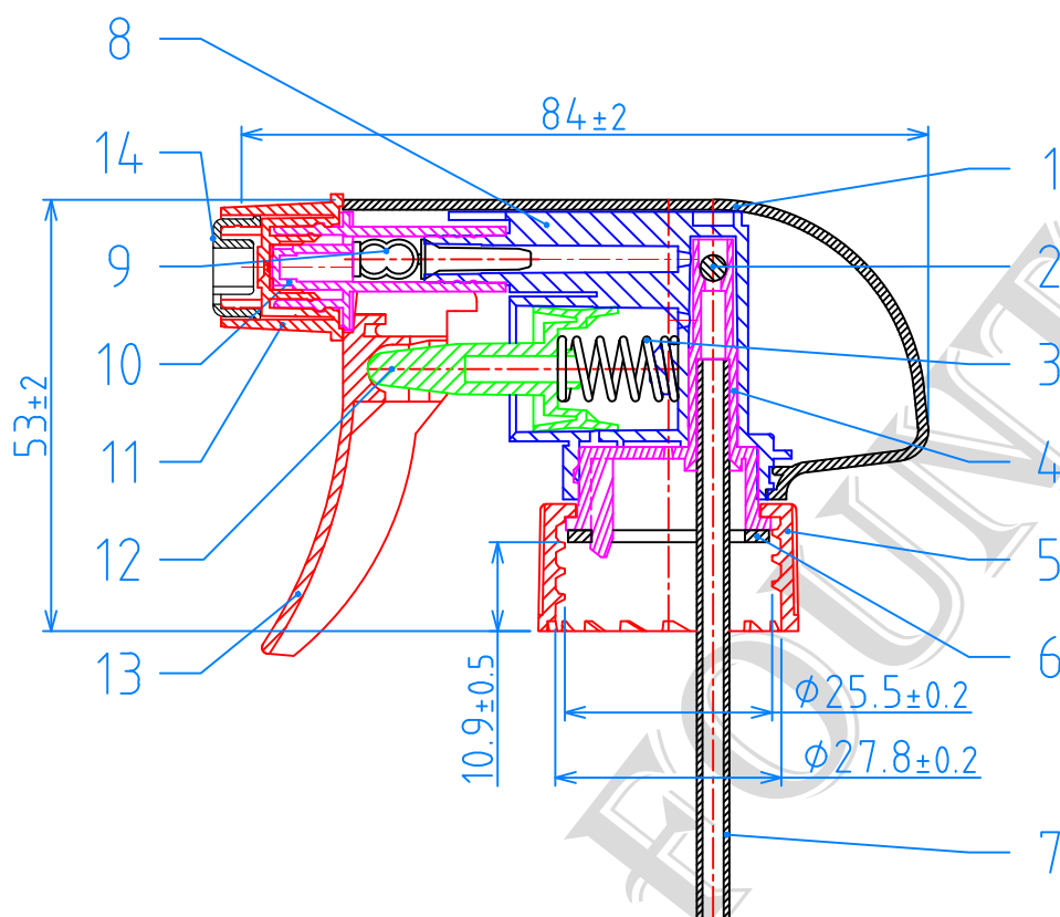
(28/410TR) CAP , P=1"x6 TPI
